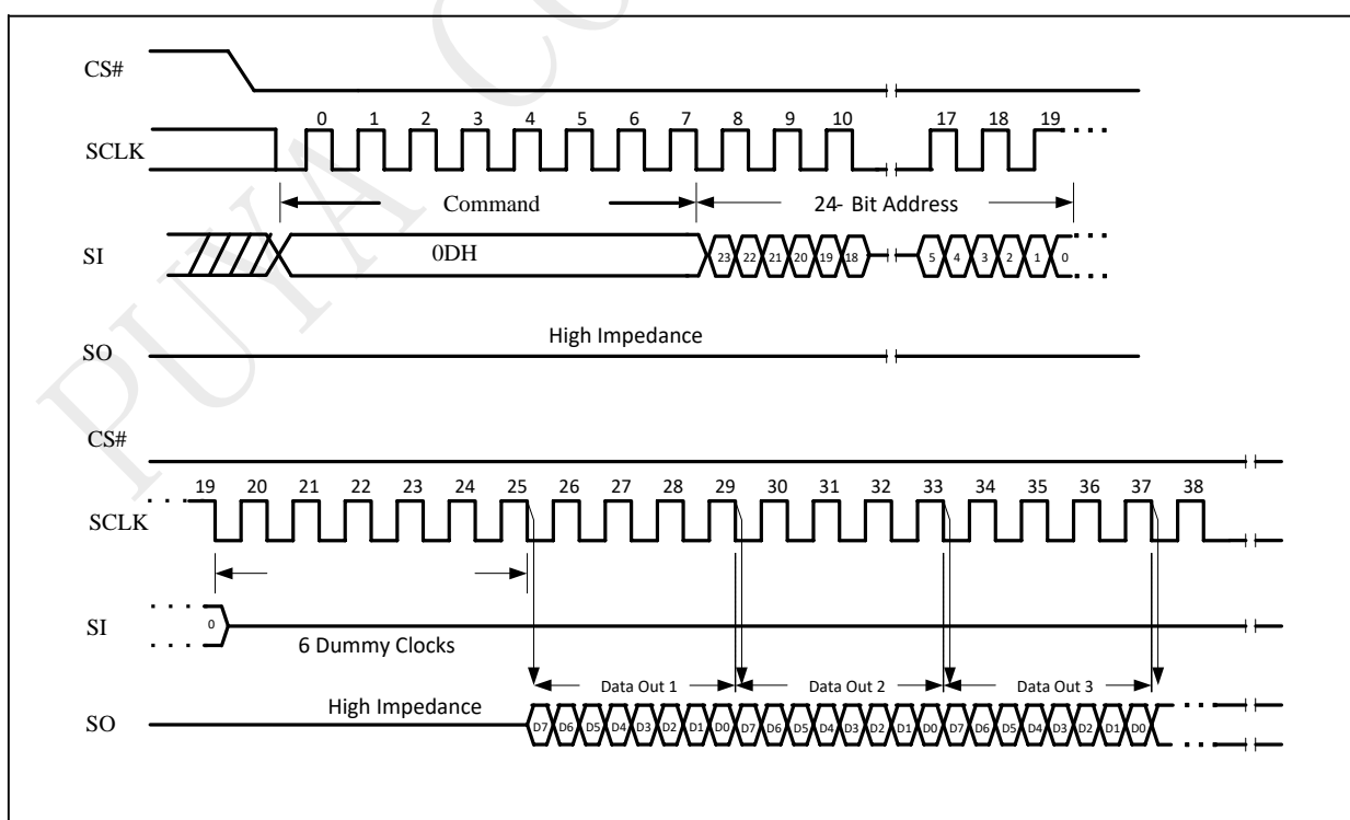
Figure 10-11 DTR Fast Read Sequence (Command 0D)
